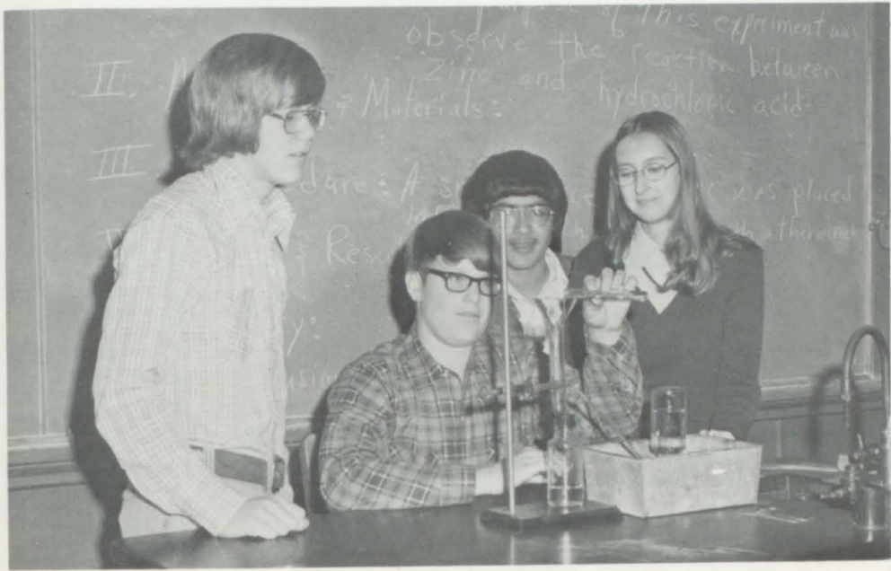
Freshman science students experiment with zinc and hydrochloric acid to discover basic properties.
